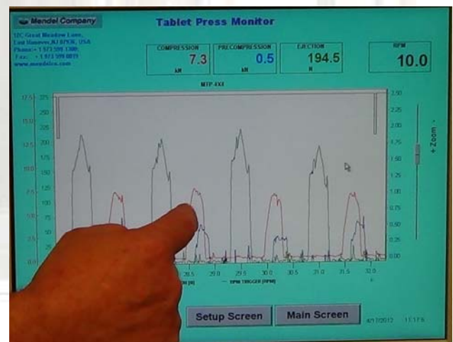
Scaled forces for Pre-Comp, Main and Ejection, with RPM
